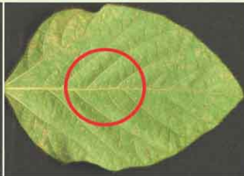
with Flutriafol
