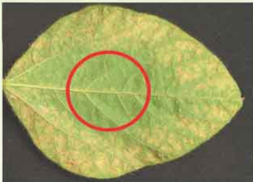
Other triazol
